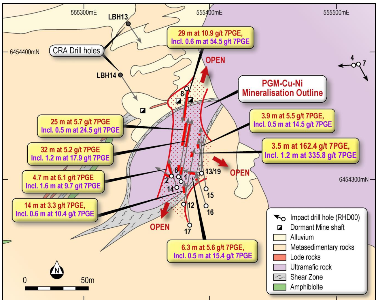
Figure 1. Drill hole location plan for Red Hill showing the location of the newly reported assay results (Drill hole details are in the ASX Releases highlighted at the start of this report).
