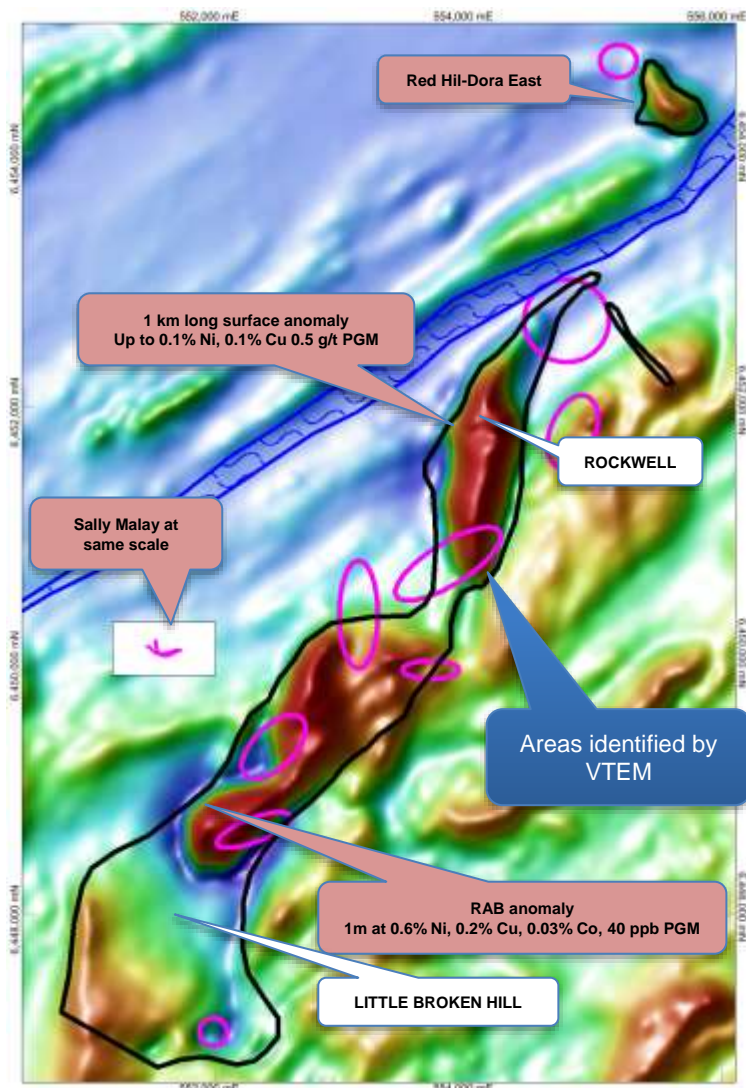
Figure 2. Image of magnetic data over the Rockwell-Little Broken Hill Trend showing areas for follow up of VTEM (pink), the interpreted outline of the mafic-ultramafic rocks in black and key exploration results.
