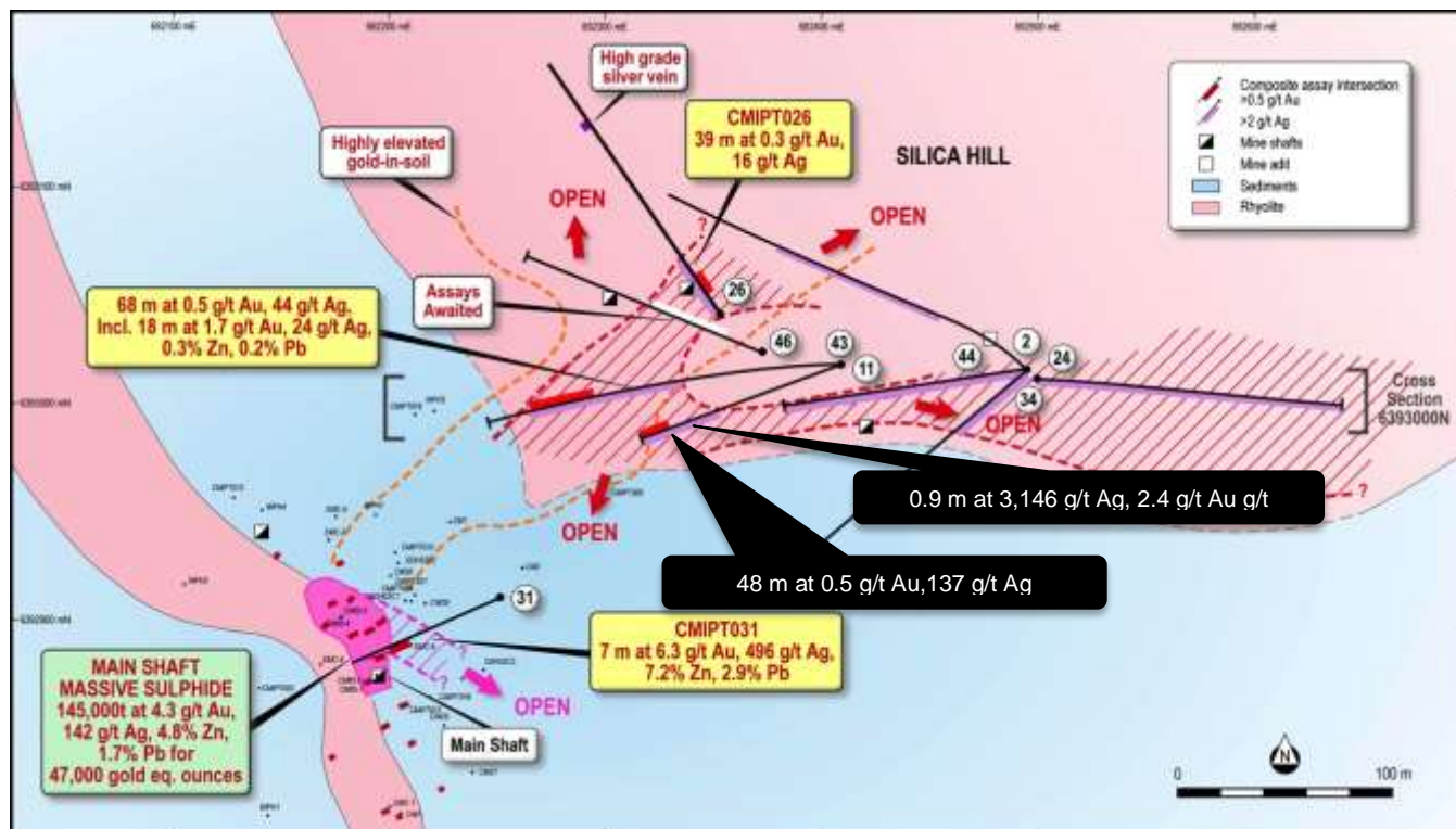
Figure 2. Surface geology map showing significant drill intercepts at Silica Hill and Main Shaft.
